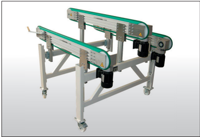
Round belt conveyor.
